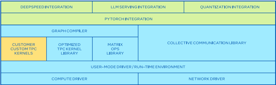
Fig 14. Intel Gaudi software stack.
