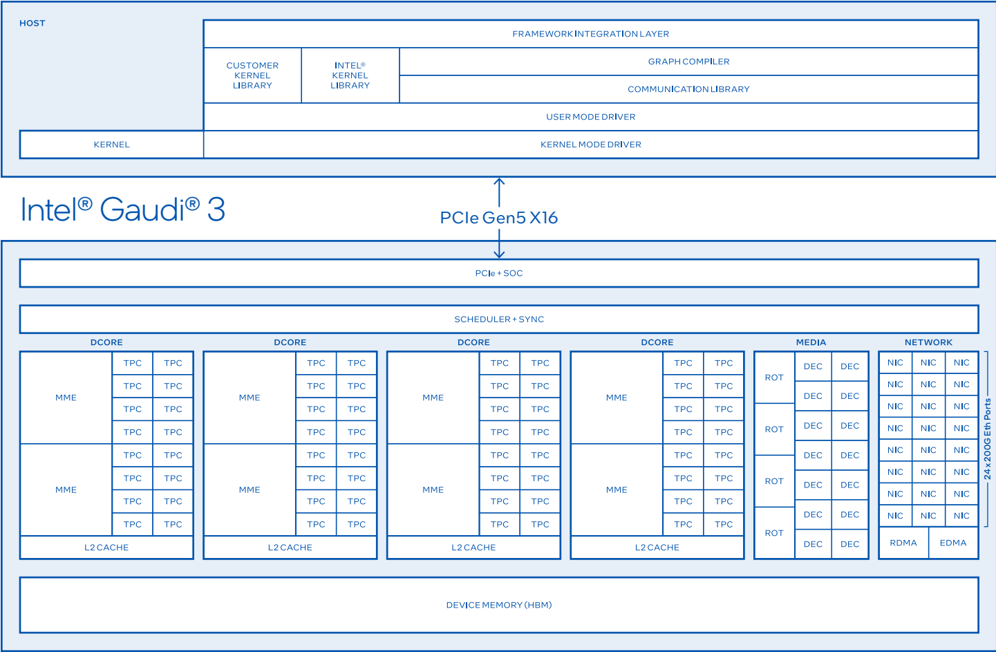
Fig 6. Intel® Gaudi® 3 architecture with DCore point-of-view and supporting software layers.
